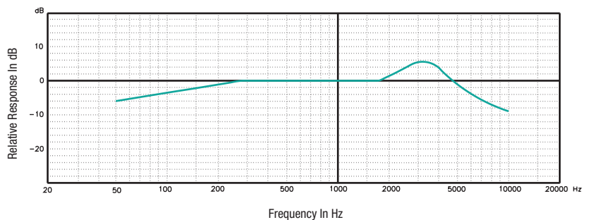
Frequency Response
