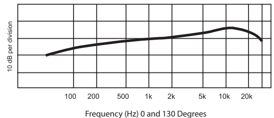
Frequency Response
